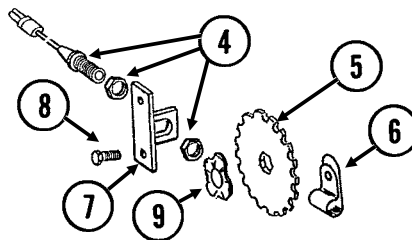
Magnetic Distance Sensor (MDS)
